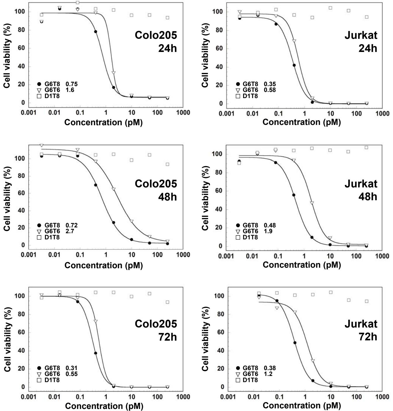
Supplementary Figure S5: G6T8 and G6T6 have similar cytotoxic activity on TRAIL-sensitive cell lines. Colo205 or Jurkat cells were treated with TRAILR2-specific tandem Tn3 proteins containing either 6- or 8-repeats of the G6 module (G6T6, G6T8), or with a negative control protein containing 8-repeats of a non-binding Tn3 (D1T8). Cell viability was assessed after 24, 48 or 72 hours by CellTiter-Glo. EC50 values for inhibition of cell viability are shown within each graph and are in pM concentrations.
