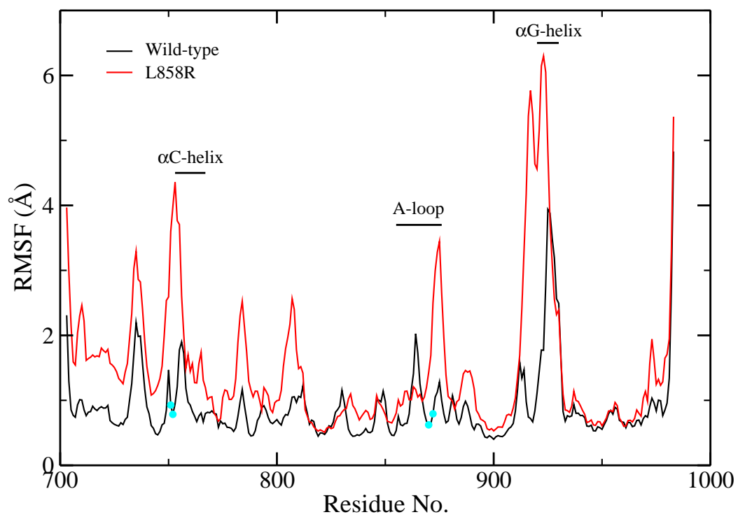
Figure S3. Backbone root-mean-square fluctuations (RMSF) from the average structures of wild-type (black line) and L858R mutant (red line) EGFRs.
