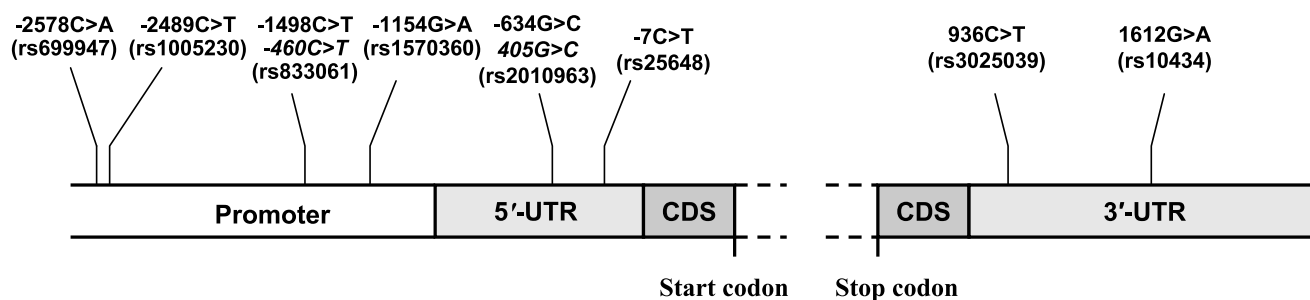
Figure 1. Structure of VEGF gene and position of VEGF SNPs relative to translation start site. Italic positions indicate alternate names. Dashed lines indicate the region consisting of coding sequence (CDS) and seven introns (adapted from ref. 29).
