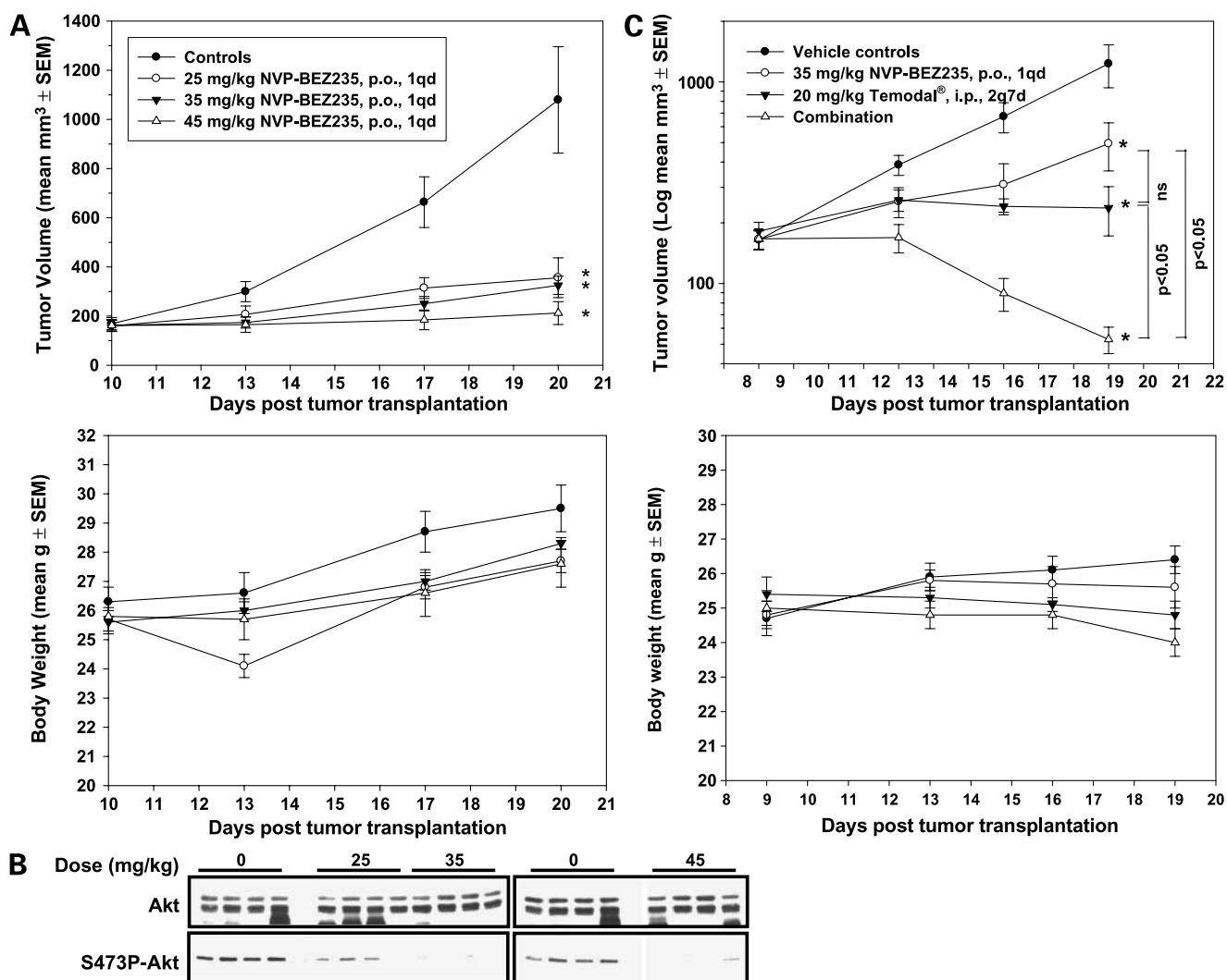
Figure 6. Effects of NVP-BEZ235 against experimental glioblastoma tumor model. U87MG tumor-bearing animals were treated with either NVP-BEZ235 alone (A–C) or in combination with temozolomide (C) at the indicated doses and schedules. Tumor volumes were callipered and body weight was measured during the course of the experiment (A and C). One hour after last dose, the animals were sacrificed and tumor was removed and analyzed as described in Fig. 5B (B). *, P < 0.05 , one-way ANOVA with Dunnett's post hoc test.
