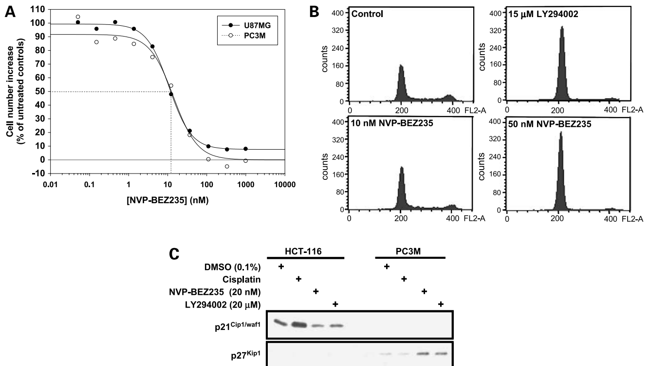
Figure 4. Effects of NVP-BEZ235 on proliferation and the cell cycle. A , U87MG and PC3M cells were incubated with increasing amount of NVP-BEZ235 for 72 h. Viable cells were then stained and cell proliferation was estimated with a standard methylene blue staining assay. Cell proliferation is expressed as a percentage of the average difference in cell number observed in NVP-BEZ235-treated cells divided by the average difference observed in untreated controls (100% represents the maximum cell proliferation observed and 0% represents the inoculum; the number of cells at the time in which the compound is added to the medium). B , PC3M cells were incubated with the indicated compound for 24 h. Determination of cell number was then determined by fluorescence-activated cell sorting. C , PC3M and HCT116 cells were incubated for 24 h with the indicated compounds. Cells were then lysed and cell extracts were analyzed by Western blotting for p21 Cip1/Waf1 and p27 Kip1 cyclin-dependent kinase inhibitors.
