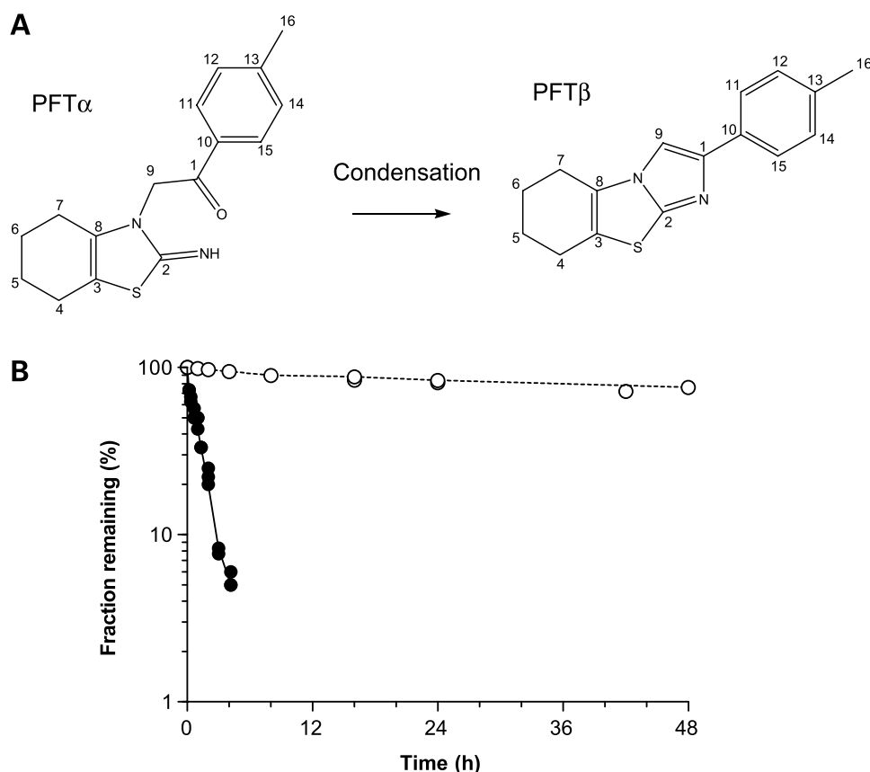
Figure 1. A , structure of PFT- \alpha and its condensation product PFT- \beta . B , stability of PFT- \alpha in DMSO at room temperature (○) and in tissue culture medium (DMEM containing 10% fetal bovine serum, 5 mmol/L L-glutamine, and nonessential amino acids) at 37°C (●). Individual data points from two independent experiments.
