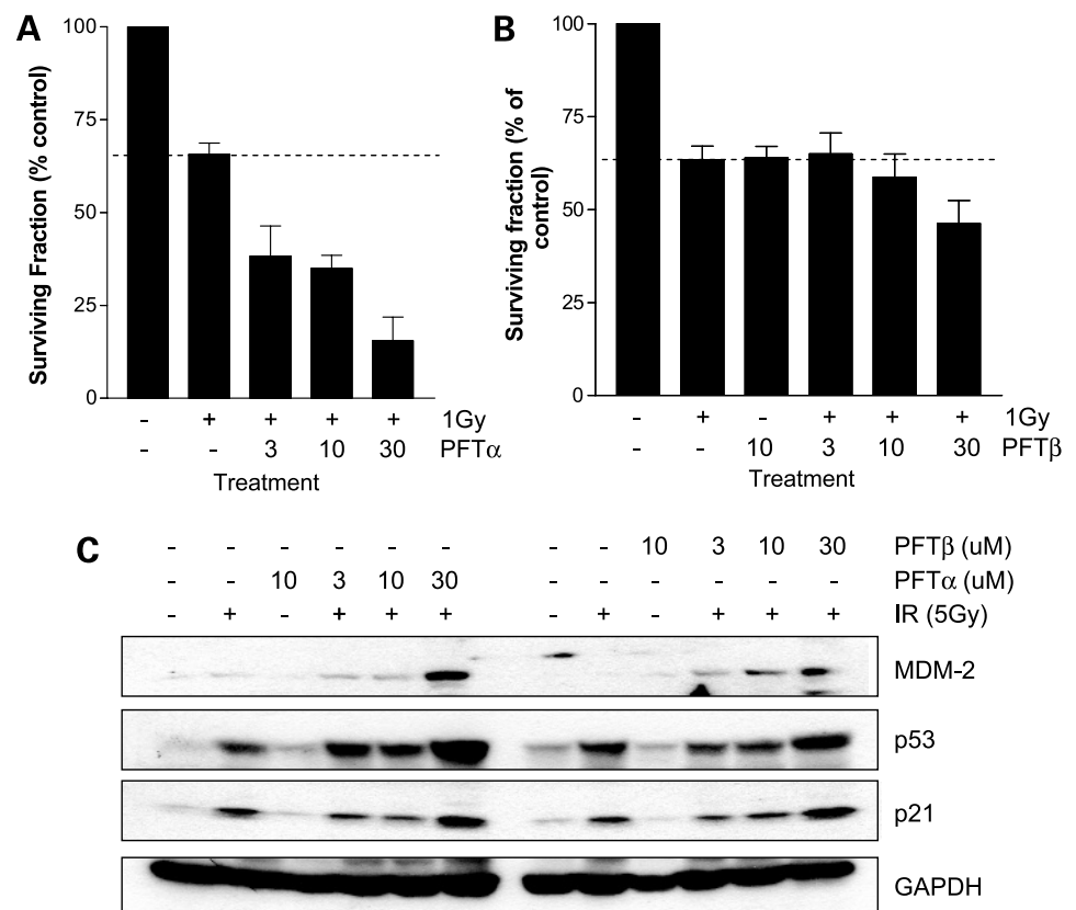
Figure 3. Clonogenic survival of A2780 cells exposed to 1 Gy of ionizing radiation alone or in combination with increasing doses of PFT- \alpha (A) or PFT- \beta (B). Values above the dotted line indicate protection, and values below the dotted line indicate enhanced cytotoxicity by PFT compounds. Bars, \pm SD. C, Western blot for MDM-2, p53, and p21 from A2780 cells treated 4 h previously with 5 Gy ionizing radiation alone or in combination with increasing concentrations of PFT- \alpha or PFT- \beta . Similar results were obtained in repeat experiments. For further details, see Materials and Methods.
