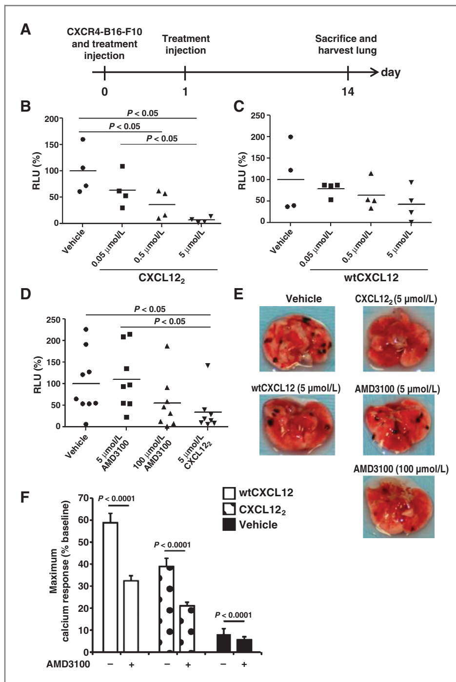
Figure 1. CXCL12 2 inhibits CXCR4-B16 metastasis more effectively than wtCXCL12 and AMD3100. A , CXCR4-luc-B16-F10 cells ( 4 \times 10^5 ) were injected intravenously into the tail vein of C57BL/6 mouse with the indicated concentrations of drugs. On day 1, the animals were given the same treatment intravenously. Lungs were harvested 14 days after inoculation, and luciferase activity was measured to evaluate metastatic tumor. CXCL12 2 ( n = 4 ; B ), wtCXCL12 ( n = 4 ; C ), and AMD3100 data (vehicle, n = 9 ; others, n = 8 ; data are a summation of 2 independent experiments; D ) are shown. E , representative lung images from mice treated with each drug are shown. F , calcium response of CXCR4-luc-B16-F1 cells induced by 500 nmol/L CXCL12 2 or wtCXCL12 was measured in the presence and absence of 5 \mu mol/L AMD3100. Experiments were recorded in quadruplicate on 2 separate days. Tumor burden was assessed by measuring luciferase-dependent light production using relative light units (RLU).
