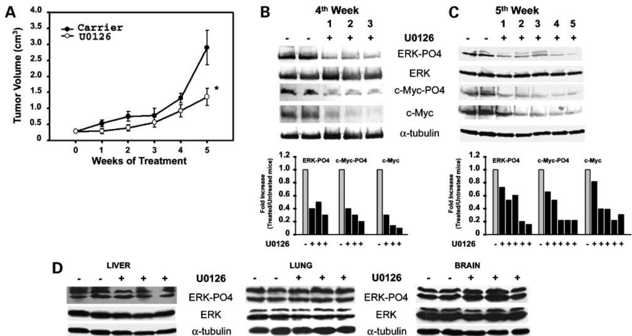
Figure 3. Tumor growth and molecular changes in untreated and U0126-treated mice. A , growth curves of xenografted RD cells. U0126 was i.p. inoculated at 25 \mu\text{mol/kg} /mouse (O—O), whereas untreated mice were inoculated with carrier solution (●—●). Mean \pm SD of tumor size of mice per group. *, P < 0.05 versus control. B , effects of U0126 in tumors 24 h post-injection in the 4th week of treatment. Left , immunoblot analysis of phospho-ERKs, total ERK, c-Myc, phospho-c-Myc, and \alpha -tubulin as loading control in tumors from treated (+) and untreated (–) mice; right , quantification of each sample of the Western blots as a fold increase of the indicated proteins in the U0126-treated mice (1–3) over the untreated mice (C) arbitrarily set at 1 (each sample was quantified as phosphorylated/unphosphorylated protein/tubulin). C , effects of U0126 in tumors 24 h post-injection in 5th week of treatment. Left , immunoblot analysis of phospho-ERKs, total ERK, c-Myc, phospho-c-Myc, and \alpha -tubulin as a loading control in tumors from treated (+) and untreated (–) mice; right , histograms obtained as in B . D , immunoblot analyses of phospho-ERKs and ERKs in normal tissue from the same treated (+) and untreated (–) mice as in B (4th week). Representative immunoblot analyses. Fold increase over the control, arbitrarily set at 1, obtained by densitometric analysis. B to D , two representative control mice (C).
